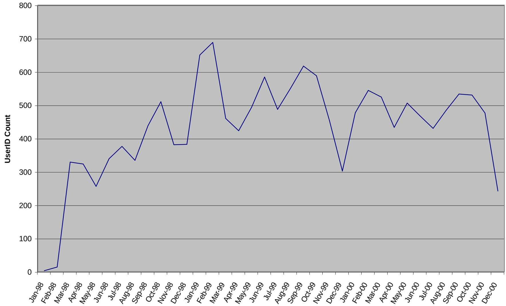
CrossFire Usage
